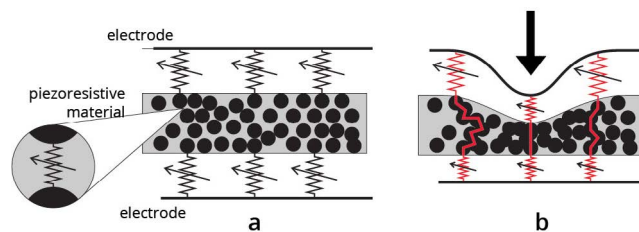
Figure 2. Illustration of the piezoresistive effect. When pressure is applied (right), the spacing between the conductive molecules is reduced and the surface contact is improved. Both effects create a measurable change in resistance.
