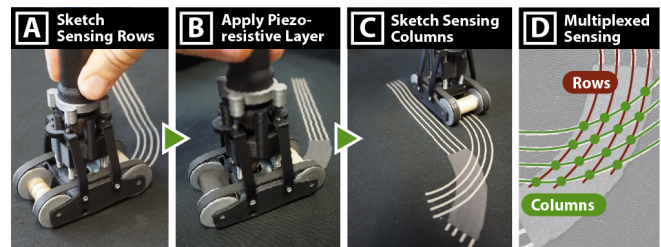
Figure 9. Pressure-Touch sensing matrix consisting of 4 \times 4 electrodes and piezoresistive fabric.
