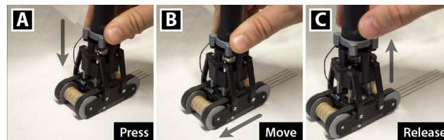
Figure 5. To create functional traces, the user has to press the material-loaded RIO device down (A), hold & move the device in the desired direction (B) and finally release the iron to finish (C).
