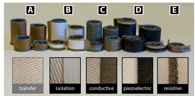
Figure 4. Different raw materials can be used for various applications. For instance, a generic transfer (A) can iron-on other materials, isolations (B) can shield or hide circuits, while conductive (C), piezoelectric (D) and resistive (E) fabric can be utilized for traces and sensors.
