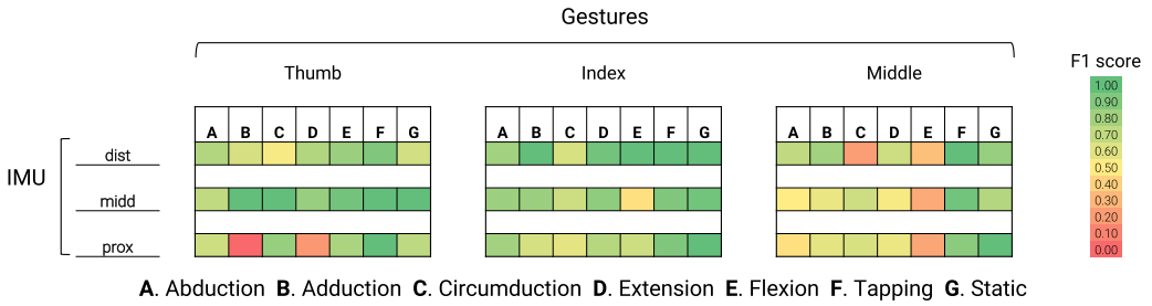
Fig. 8. F1 score of single IMU models trained for multi-class classification. The classes include six different gesture types possible with each finger (+1 static) for each model during Freehand microgestures. Note that different models were trained with IMU on each segment (distal, middle, proximal) and for different gesturing fingers.
