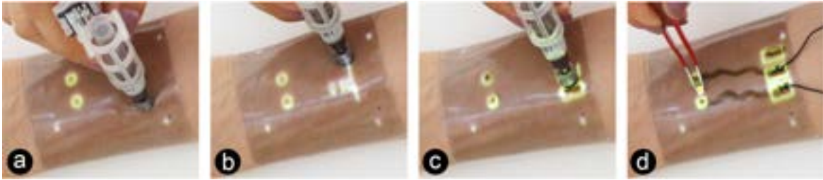
Figure 3.9 Placing electronic components. The user defines the location of a component's pad (a) and then drags the pen to define the distance and orientation of other pads (b). The system displays the footprints and the user starts inking (c). Finally, the user connects components using bare conductive (d).
