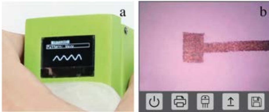
Figure 4.5 Print-A-Sketch user interface: (a) the user controls most functionality directly on the hand-held tool (here: selecting the trace pattern), (b) the backend interface supports additional functionality (e.g., showing the live camera view).
